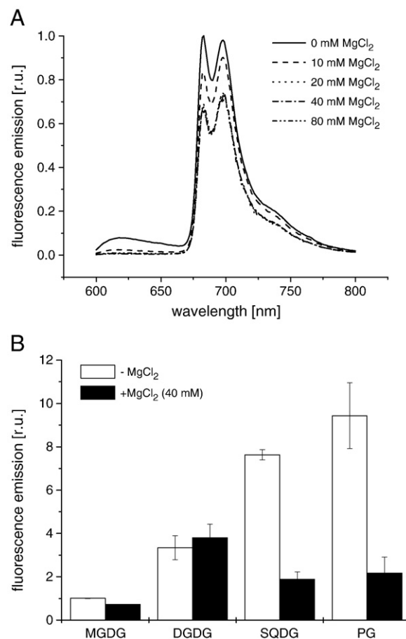
Fig. 4. A) 77K fluorescence emission spectra of LHCII samples in the absence or presence of \text{MgCl}_2 which was added at the final concentrations of 10, 20, 40 and 80 mM, respectively. The pH was kept constant at a pH of 7.8. The spectra are shown in relation to the normalized maximum fluorescence emission value of the control sample without \text{MgCl}_2 (which was normalized to the value 1). Fig. 4A shows the result from a typical measurement, three independent experiments confirmed the data depicted in the figure. B) Influence of the addition of 40 mM \text{MgCl}_2 on the 77K fluorescence emission maximum of the LHCII samples incubated with MGDG, DGDG, SQDG and PG at pH 7.8. The fluorescence maxima were compared to lipid incubated LHCII samples without addition of \text{MgCl}_2 . The final concentration of the LHCII samples was 5 \mu\text{g Chl mL}^{-1} and the lipids were used at a lipid/Chl ratio of 16. The maximum fluorescence emission value of the control LHCII without lipids was normalized to 1 and the relative amplitudes of the emission maxima of lipid incubated LHCII samples are shown in relation to the normalized control value. Fig. 4B shows the mean values of three independent experiments, the standard deviations are depicted as error bars.
