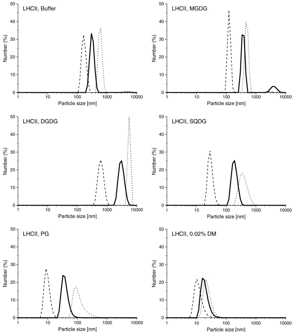
Fig. 5. The distribution of particle sizes [nm] of LHCII in Tricine buffer, lipid incubated LHCII samples and LHCII solubilized with 0.02% DM, at pH 7.8 and in the absence of additional \text{MgCl}_2 , measured by photon correlation spectroscopy (PCS). For incubation the lipids MGDG, DGDG, SQDG and PG were used at a lipid/Chl ratio of 16. The final concentration of the LHCII samples was 5 \mu\text{g Chl mL}^{-1} . Fig. 5 shows the results of three independent experiments where each sample was measured 6–12 times, depending on the reproducibility of the measurement and heterogeneity of the sample. The bold lines show the average particle sizes, dashed and dotted lines stand for the minimal and maximal measured particle sizes, respectively.
